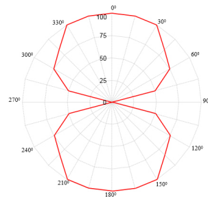
Read range (%) at various angle
